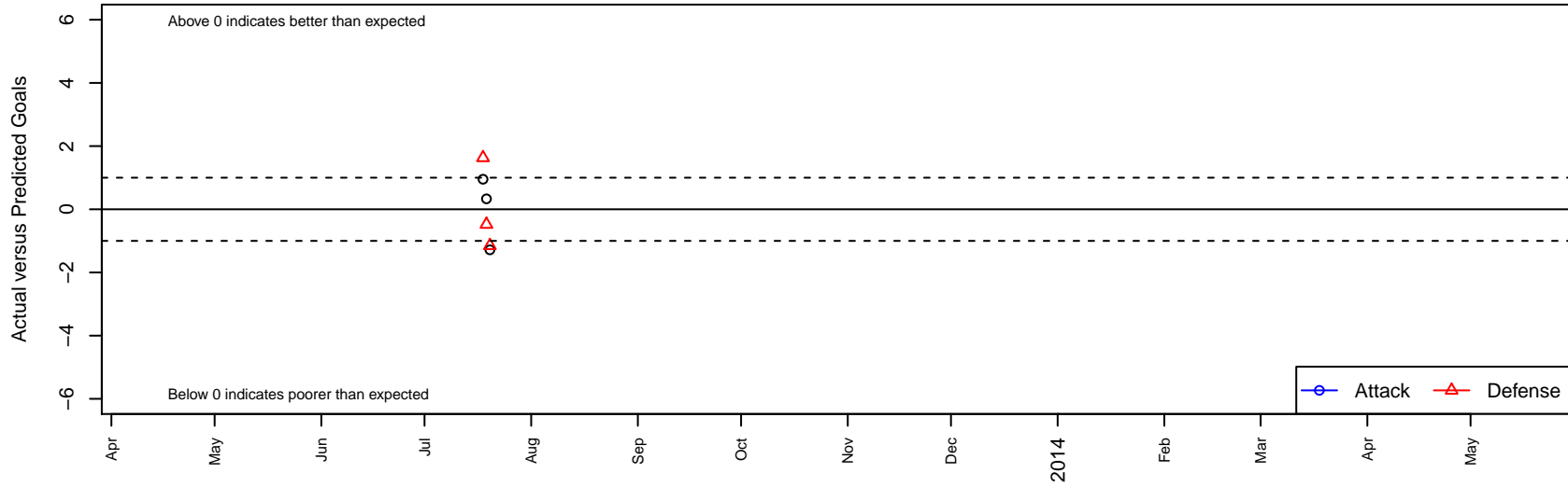
Parsippany SC B99 Dots are actual minus expected GF (blue circles) and GA (red triangles). Blue line is smoothed change in attack strength. Red is smoothed change in defense strength.
